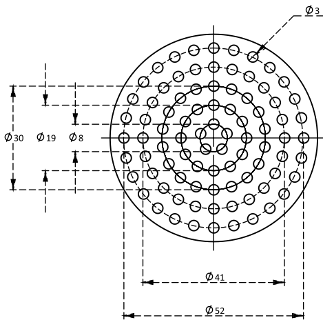
A Mechanical version Solid base
